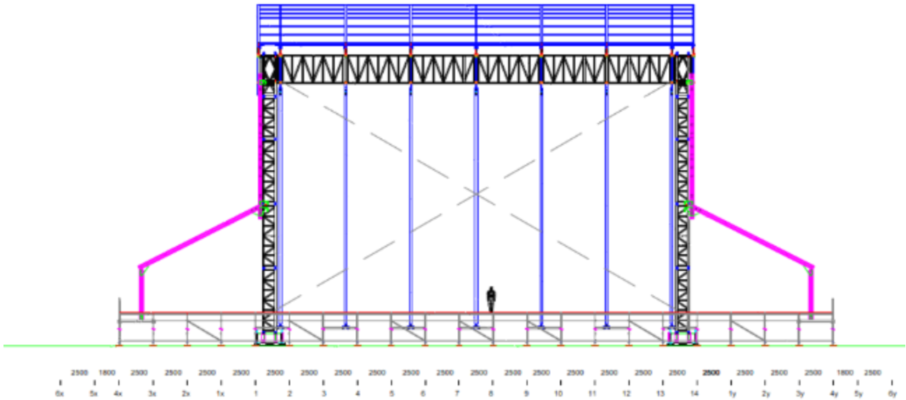
Back elevation
