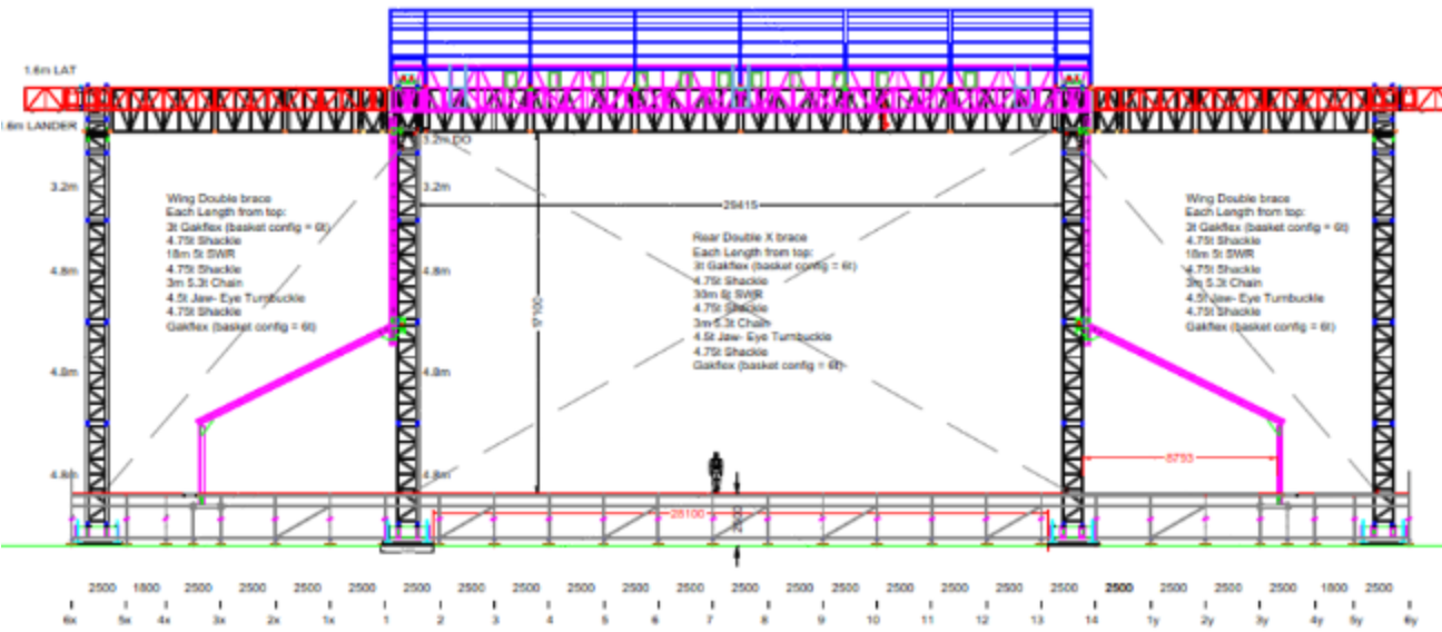
Front elevation
