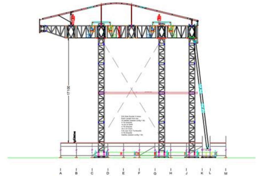
Side elevation SL
